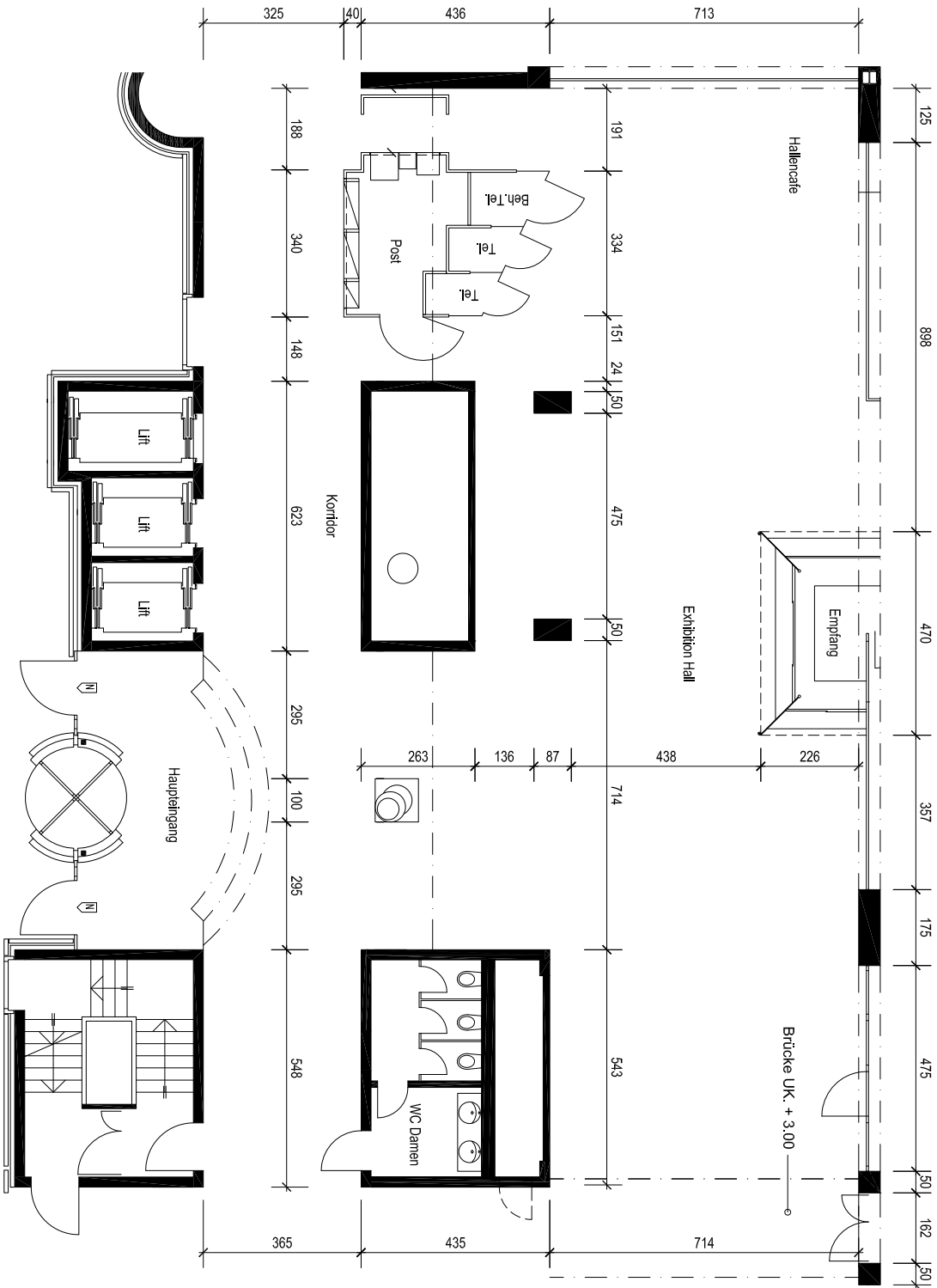
Anschlussplan: Exhibition Hall
